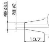
N3-20 Nozzle Size \Phi 2.0
