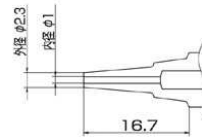
N3-23 Nozzle Size \Phi 2.3
