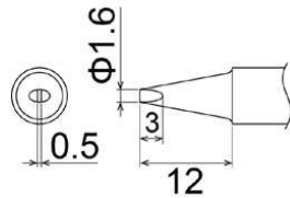
T22-D16 Shape-1.6D
