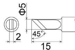
T22-K Shape-K
