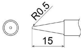
T22-BL2 Shape-2BL
