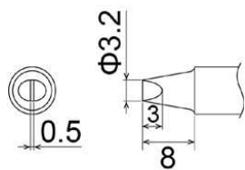
T22-D32 Shape-3.2D
