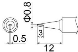
T22-D08 Shape-0.8D
