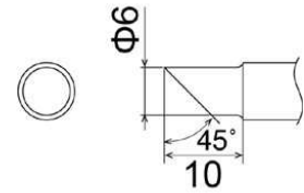
T22-C6 Shape-6C
