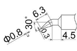
T22-JD08 Shape-0.8JD
