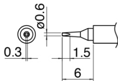
T30-D06 Shape-0.6D
