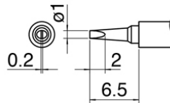
T30-D1 Shape-1D
