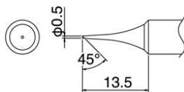
T18-C05 Shape-0.5C B3664 Nozzle assembly C
