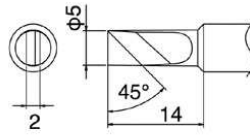
T18-K Shape-K B3665 Nozzle assembly D
